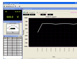
Software
